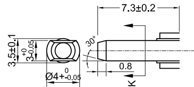
DIMENSIONS OF LEVER
