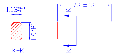
DIMENSIONS OF LEVER
