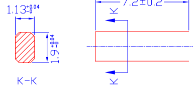
DIMENSIONS OF LEVER
